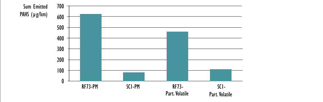
Figure 14: Effect of Fuel PAH on Emissions of PAH
